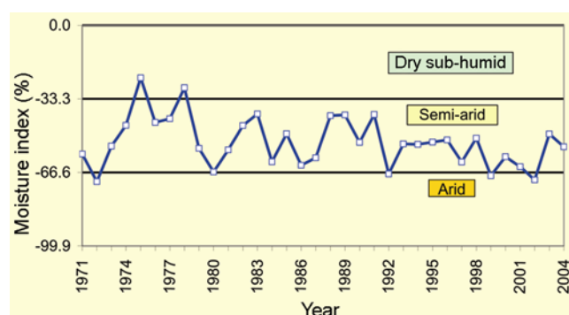
Figure 1. An illustration of climate change in Nalgonda District, Andhra Pradesh, India (source: Rao and Wani 7 ).
