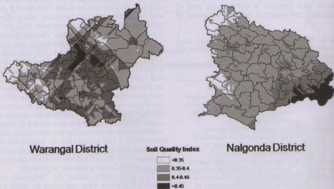
Figure 3. Soil quality index for Warangal and Nalgonda districts.
