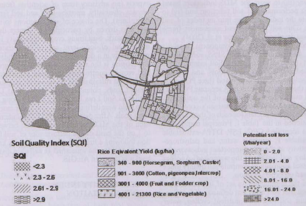
Figure 2. Thematic map for soil quality index, productivity and potential soil loss of the watershed.
