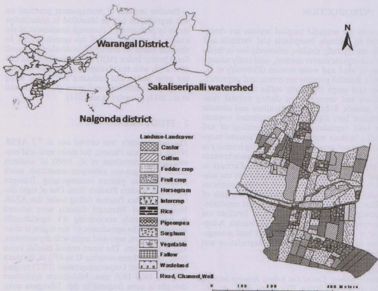
Figure 1. Land use land cover in Sakaliseripalli watershed.
