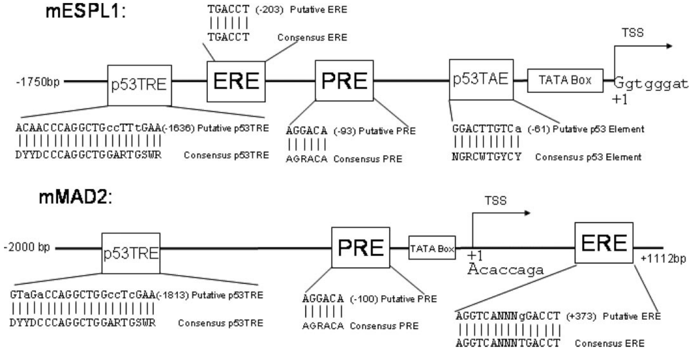
Fig. 8. Schematic drawing showing the putative sequence motifs of the separase and Mad2 promoters. Arrow, the predicted transcription start site (TSS); and C, the +1 position. T ATAT TATA-box at -30, putative progesterone responsive element (PRE), estrogen responsive element (ERE), p53 transcriptional activation element (p53TAE) and p53 transcriptional repressor elements (p53TRE) are also shown. The following IUPAC-IUB codes for nucleotides were used: R, purine (A or G); Y, pyrimidine (C or T); W(A or T); S(G or C); D (G, A, or T); N, any nucleotides.
