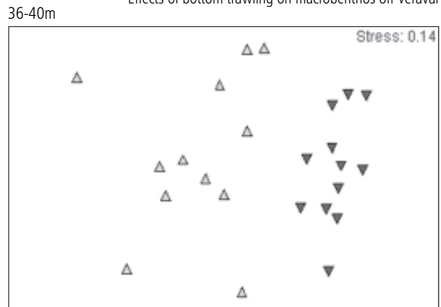
Fig. 4. MDS plots for total macrobenthos during September 2005 to November 2006
