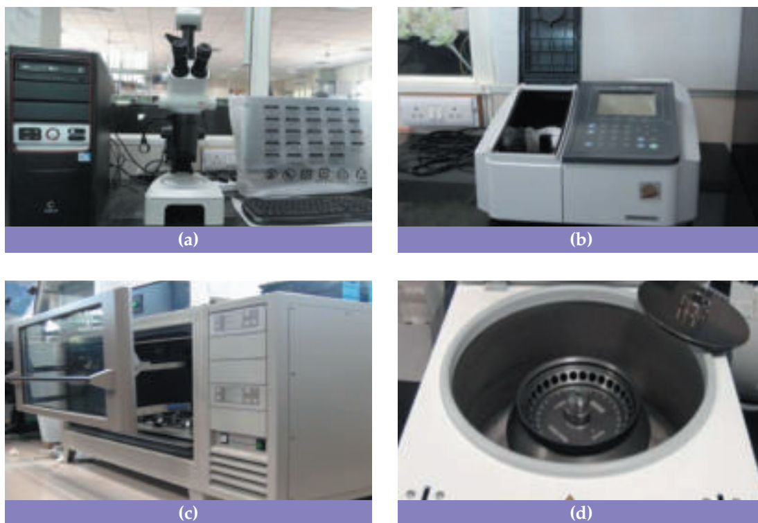
Fig. 2.3. Recently procured Leica-Stereomicroscope and imaging system (a), Shimadzu-UV/Vis Spectrophotometer (b), Khuner-Refrigerated incubator shaker (c) and Hettich-Refrigerated centrifuge (d)
