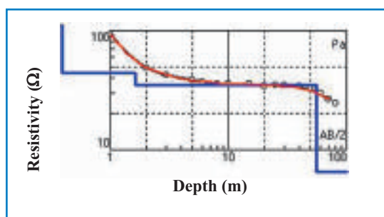
Fig. 3.13. Electrical resistivity data output at location 2 of NIASM site
