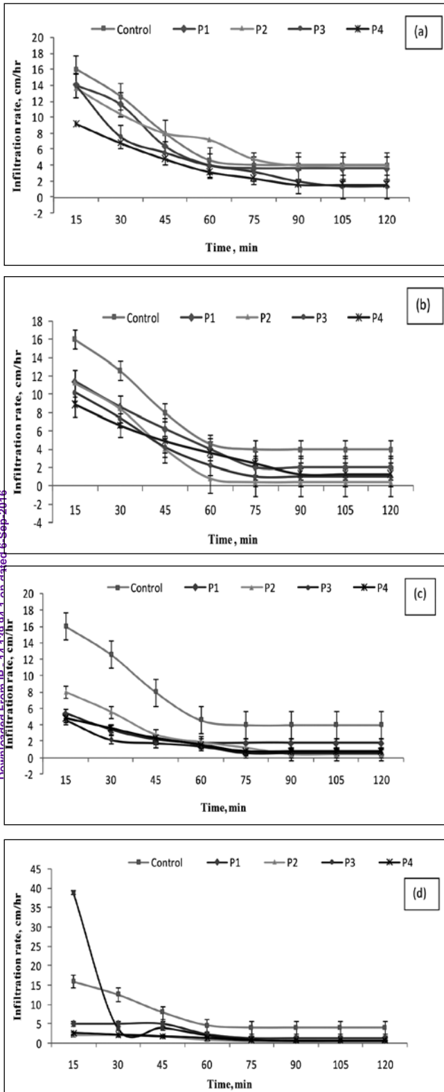
Fig. 1 : Infiltration characteristics of sandy loam soils with selected super absorbent polymers under different concentrations minimum was in P1 (65%) during steady state condition. It is observed that, the percentage reduction increased as polymer concentration increased from 0.25 to 1.75%. Shane Phillips (2007) showed that PAM-1011 can significantly reduce
