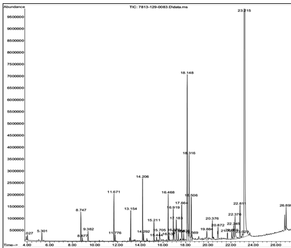
Figure 5. GC-MS chromatogram of the crude ethyl acetate extract of U. fasciata .
