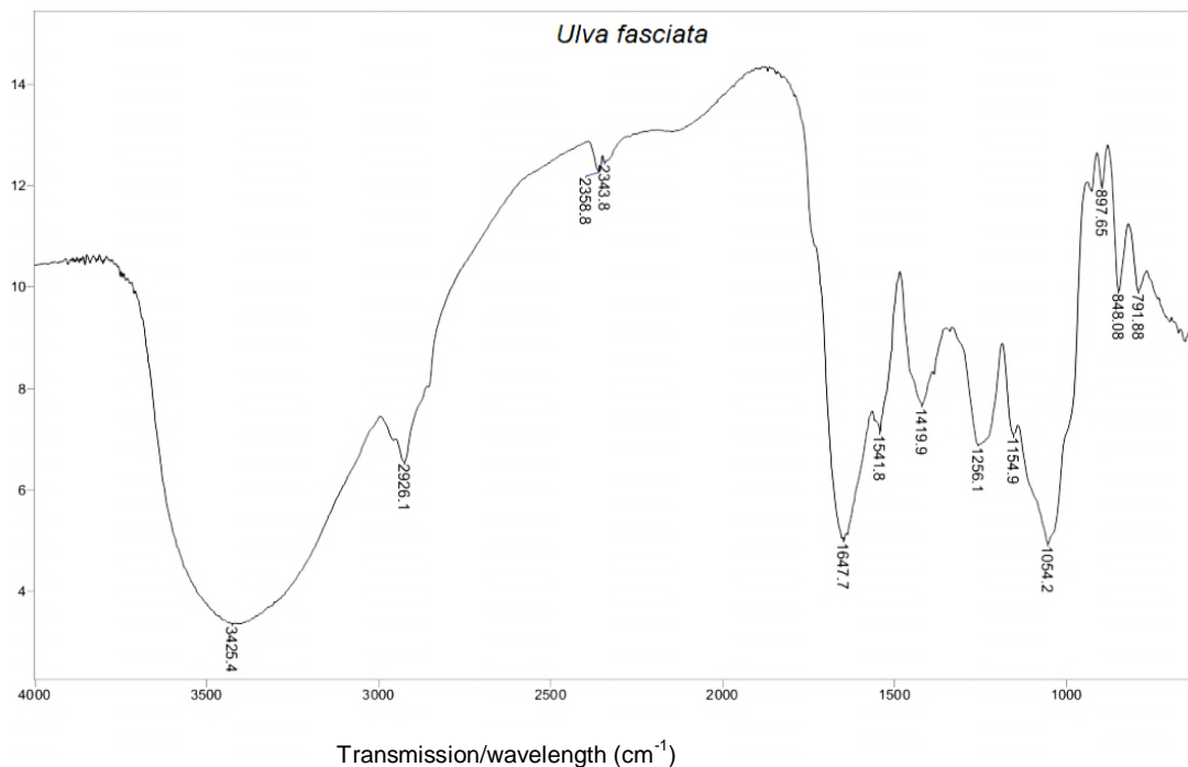
Figure 4. FTIR spectrum of shadow dried powder of U. fasciata .
