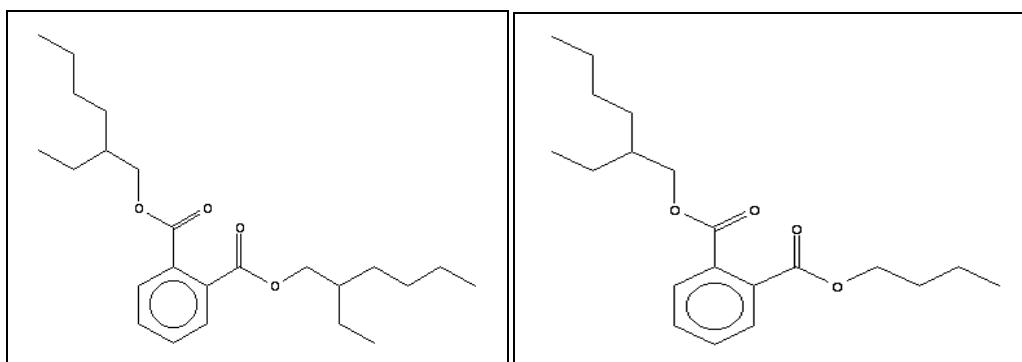
Figure 6. Major compounds isolated from U. fasciata . (a) Structure of Bis(2-ethylhexyl)phthalate ( C_{24}H_{38}O_4 ) extracted and detected by GC-MS from U. fasciata (b) Structure of 1,2-benzenedicarboxylic acid, butyl 2-ethylhexyl ester ( C_{20}H_{30}O_4 ), extracted and detected by GC-MS from U. fasciata .
