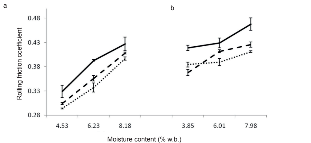
Fig. 3. Rolling friction coefficient of: a – coconut milk residue flour and b – VCO cake flour. Explanations as on Fig. 2.
