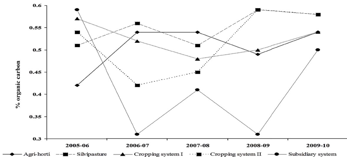
Fig. 1. Soil organic carbon status of soil (over the years) in different systems of the IFS model
