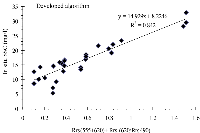
Fig. 5. Linear regression fit between in situ suspended sediment concentration (SSC) and remote sensing reflectance (R rs ) measurements used for the development of the regional algorithm.
