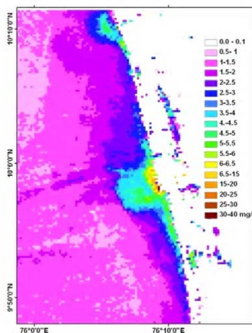
Fig. 6. Distribution of suspended sediment concentrations (SSCs) derived from the ocean colour monitor (OCM) sensor onboard Oceansat-2 (acquired on January 20, 2011) along the southwest coast of India, employing the developed regional algorithm.
