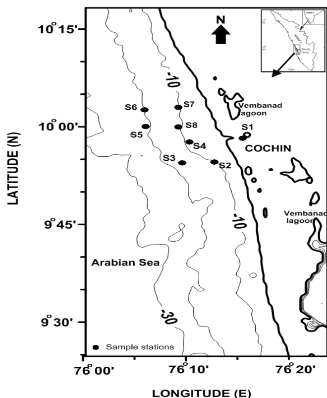
Fig. 1. Map showing the study area off Cochin, southwest coast of India. Sample stations for in situ suspended sediment concentrations (SSCs) and reflectance measurements are also shown.
