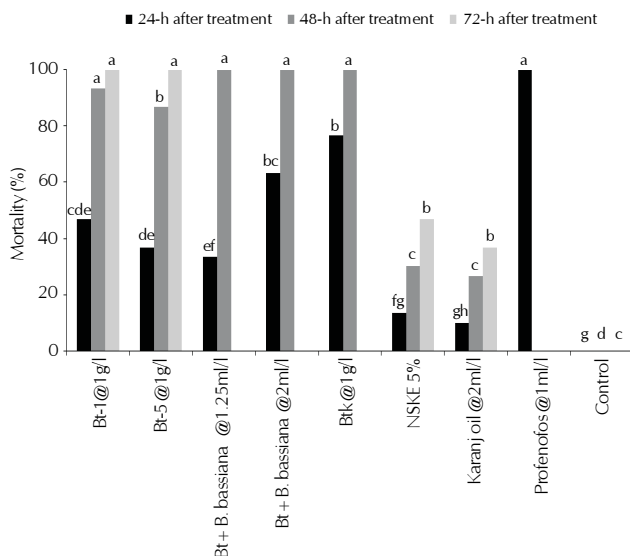
Figure 1: Laboratory evaluation of microbial, botanical and chemical insecticides against 3 rd instar larvae of semilooper ( A. janata )
