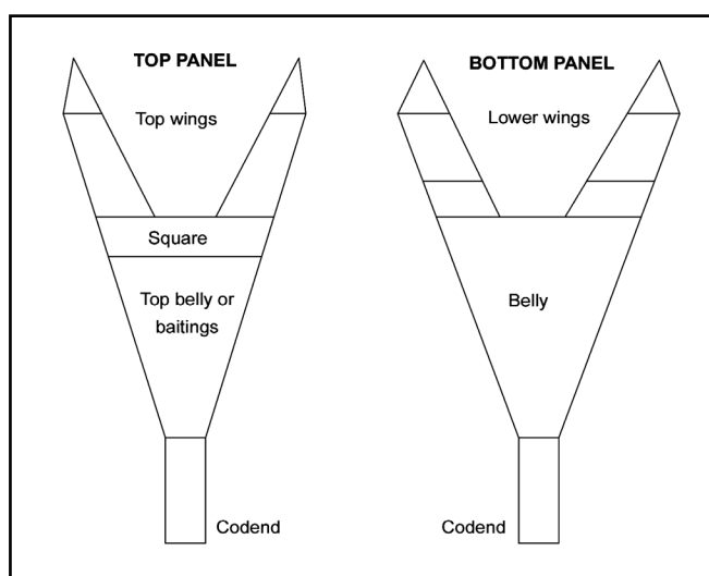
Fig. 2. Basic trawl design illustrating constituents of netting panels
