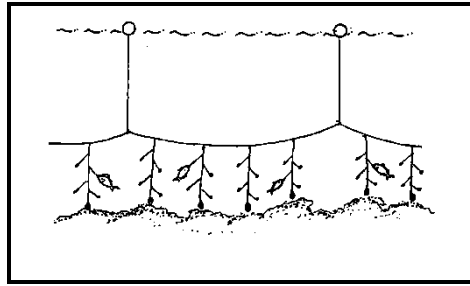
Fig. 39. Bottom vertical long line
