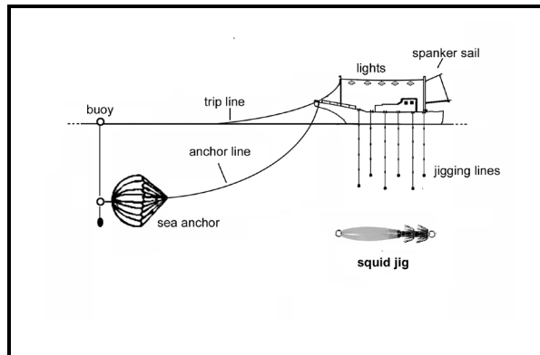
Fig. 23. Squid jigging
