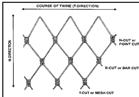
Fig. 4. Types of cuts used to shape netting
