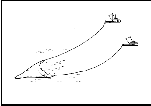
Fig. 15. Two-boat bottom otter trawl
