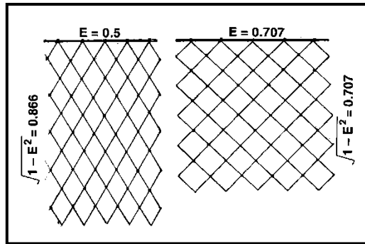
Fig. 6. Effect of different hanging coefficients on shape of netting
