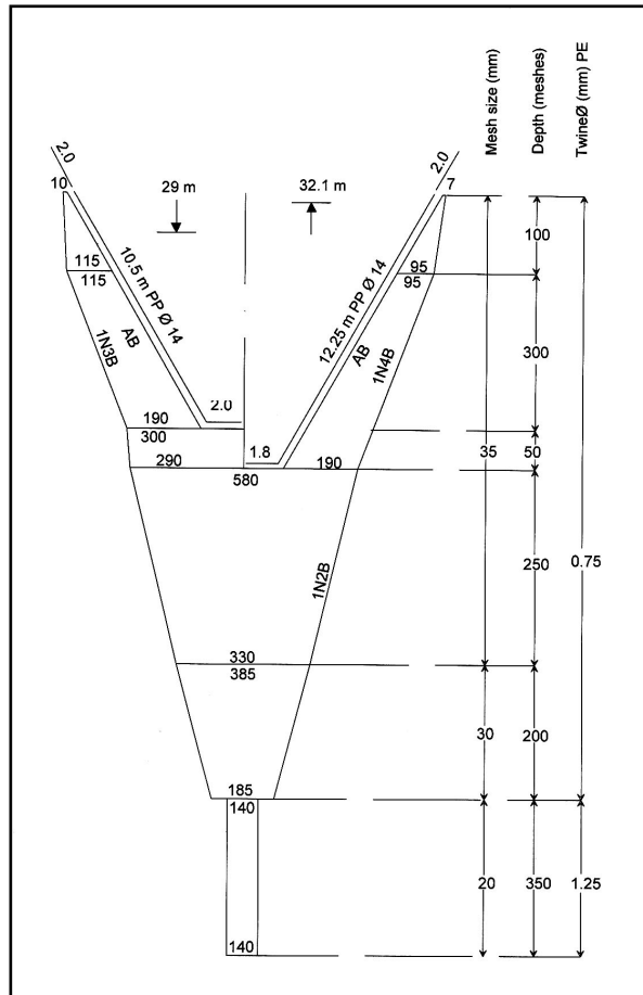
Fig. 3. Design of a 29 m shrimp trawl
