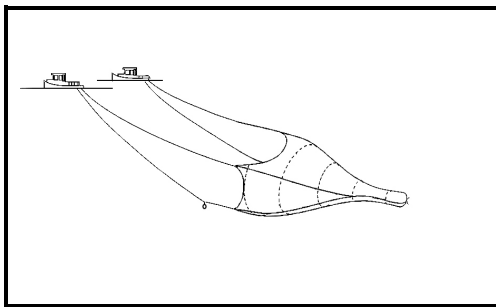
Fig. 17. Two-boat midwater trawl
