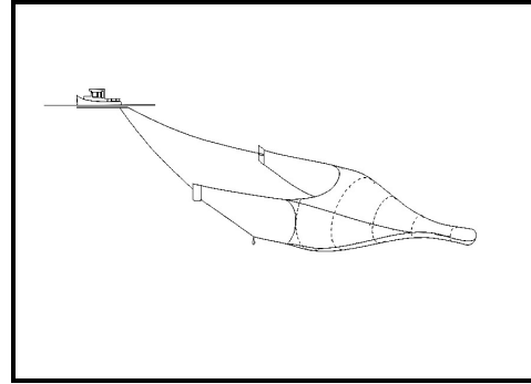
Fig. 16. One-boat midwater trawl
