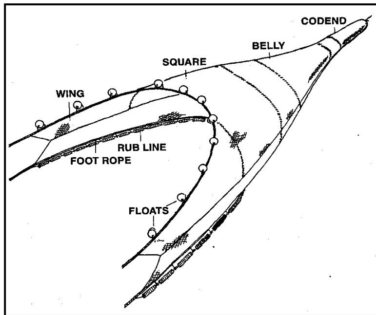
Fig. 8. Pictorial view of a two-seam demersal trawl
