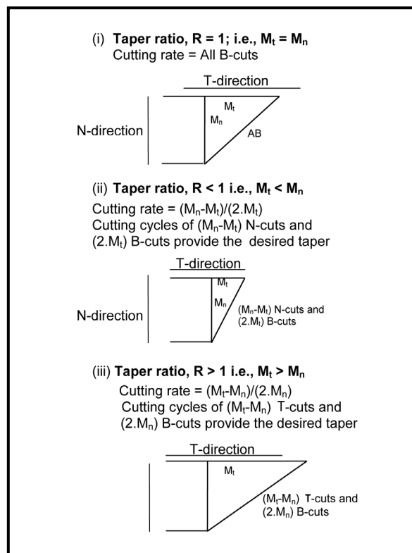
Fig. 5 Calculation of cutting rates
