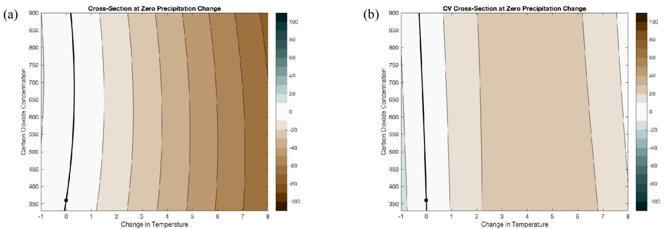
Fig. 3: Simulated (a) soybean grain yield and its (b) coefficient of variation, as affected with changes in temperature and CO 2 concentration, without changes in rainfall.
