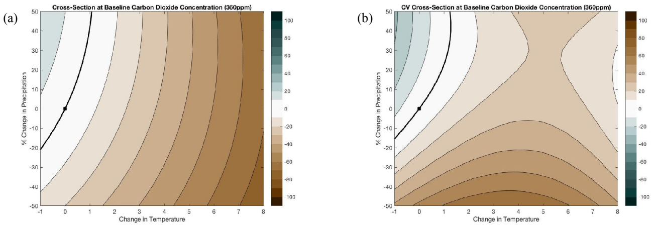
Fig. 2: Simulated (a) soybean grain yield and its (b) coefficient of variation, as affected with changes in temperature and rainfall at constant CO 2 concentration (360ppm).
