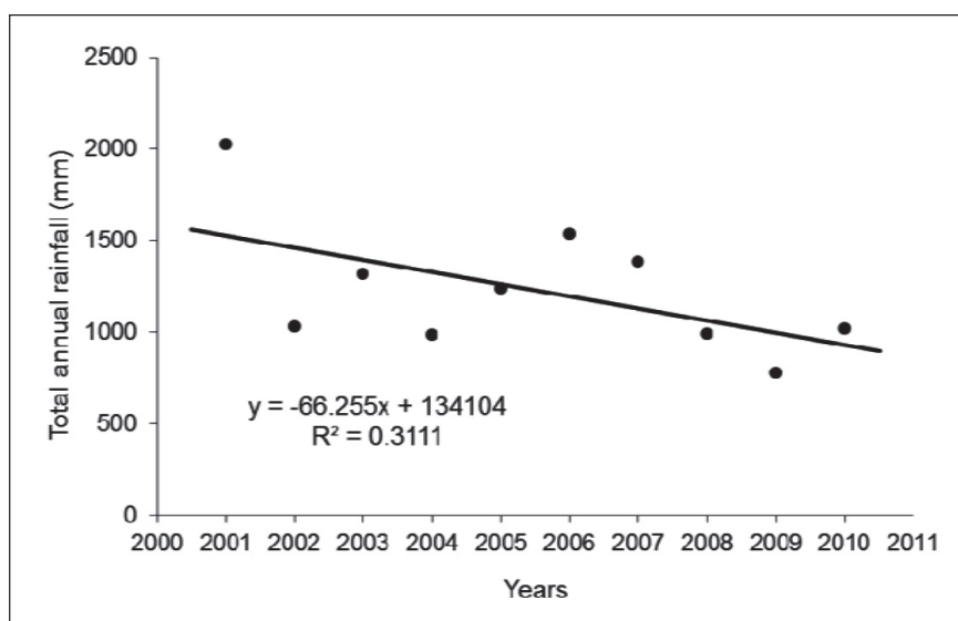
Fig 3. Trend of annual rainfall during 2001-2010 at Bamra
