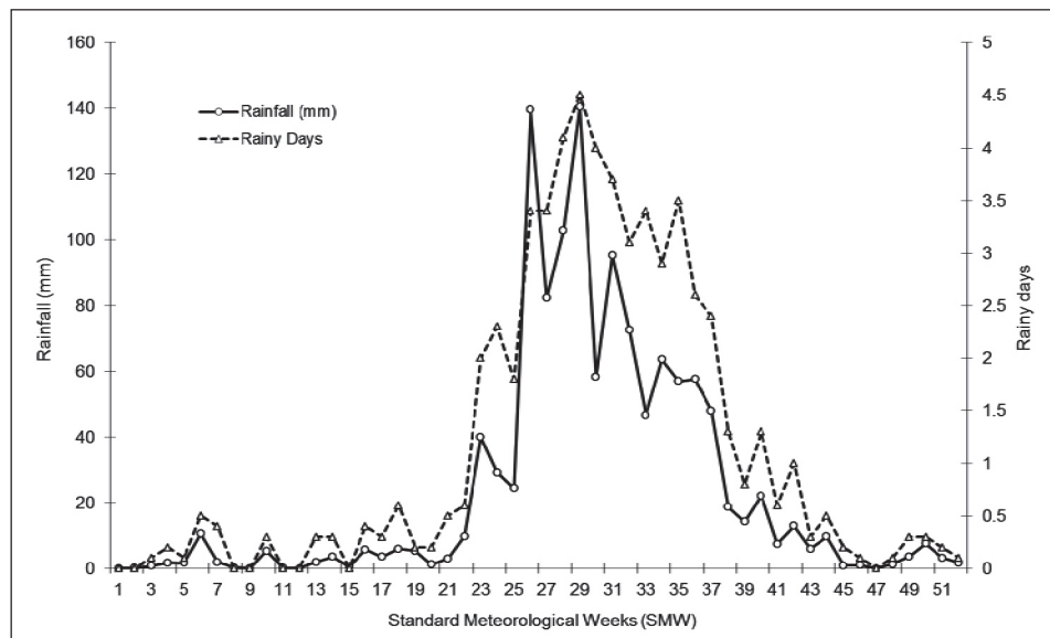
Fig 4. Weekly distribution of rainfall and rainy days at Bamra, Sambalpur, Odisha
