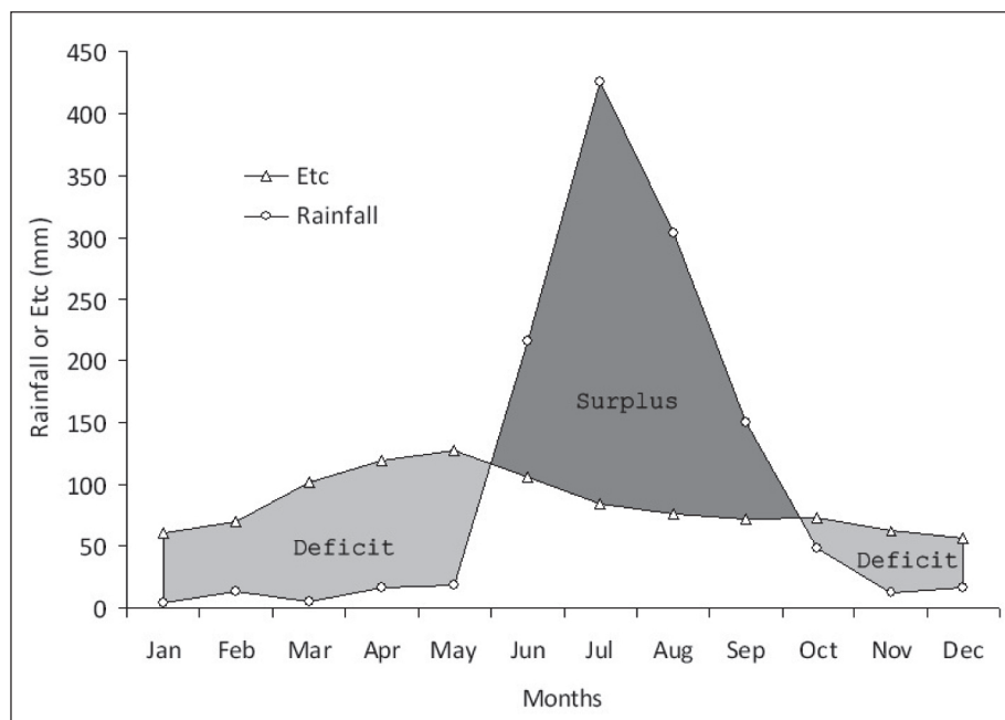
Fig. 6. Water balance of sisal crop at Bamra, Sambalpur, Odisha
