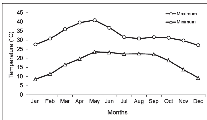
Fig 1. Mean maximum and minimum temperature during 2001-2010 at Bamra
