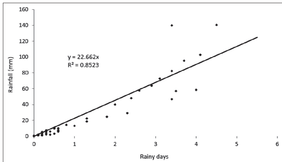
Fig 5. Relation between weekly rainy days and rainfall at Bamra, Sambalpur, Odisha
