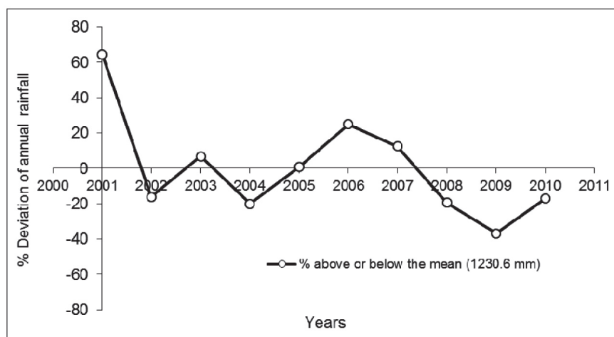
Fig. 2. Deviation (%) of annual rainfall over 10 years from the mean (1230.6 mm) at Bamra
