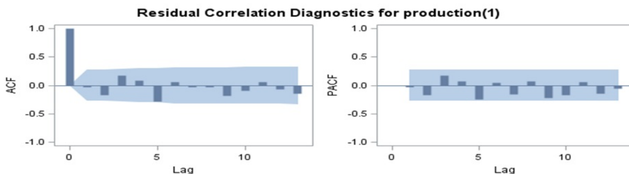
Fig. 5. ACF and PACF of the residuals of fitted ARIMAX model
