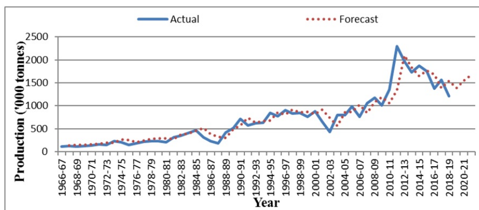
Fig. 6. Castor production ('000 tonnes) in India actual and forecasted data from the year April 1966-67 to 2021-22
