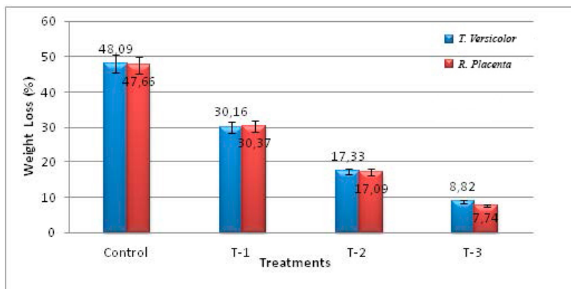
Figure 1: Effect of microwave treatment on weight loss of Bamboo blocks/samples.
