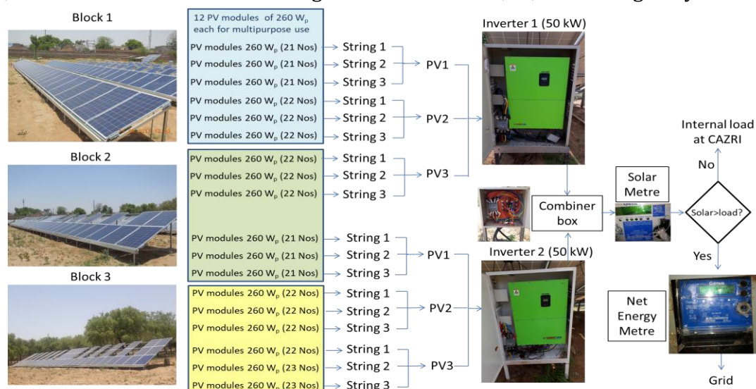
Fig. 5. Schematic diagram of PV based electricity generation in AVS and its supply to local grid.
