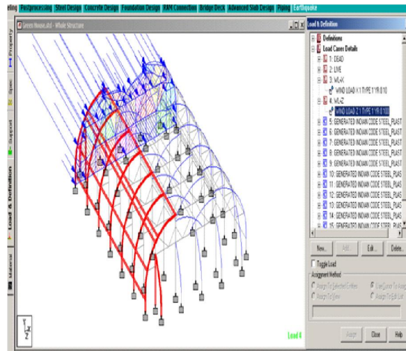
Fig. 4 Wind load in Z direction
