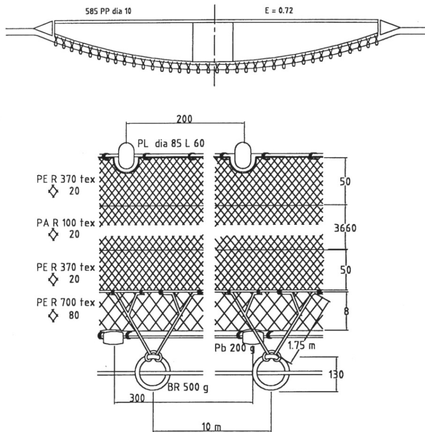
Fig. 2. Details of ring seine design and rigging
