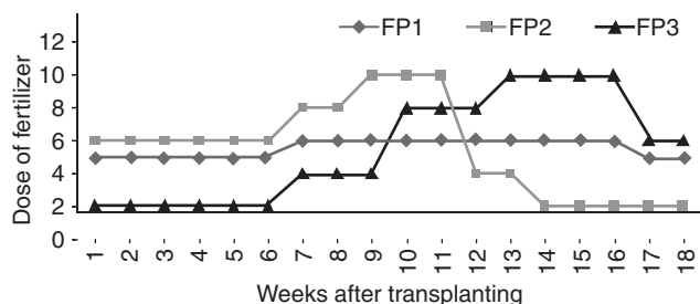
Fig 1 Fertigation schedule of tomato for total fertilizer dose of 120:60:60 NPK kg/ha.
