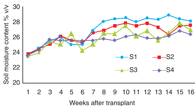
Fig 2 Soil moisture dynamics under different planting geometries.
