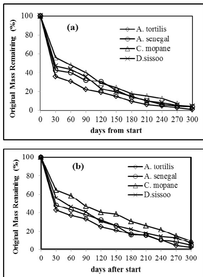
Figure 1 : Mass remaining (as percent of initial) through time for leaf litters of various MPTs incubated at (a) 100% Field capacity (b) 50 % Field capacity
