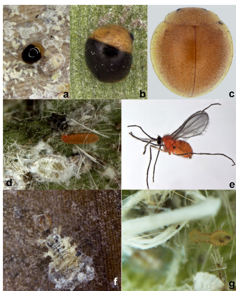
Fig. 3. Predators of Aleurodicus rugioperculatus : a, b. Cybocephalus sp.; c. Jauravia pallidula (Motschulsky); d. Larva of Diadiplosis sp.; e. Adult of Diadiplosis sp.; f. Larva of Pseudomallada sp.; g. Indet. psocid feeding on whitefly.
