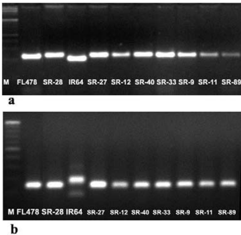
Fig. 6.3: SSR polymorphism using Saltol markers, a. RM10694, b. RM8094 in parents and salt-tolerant introgression lines from IR64/FL478 cross
