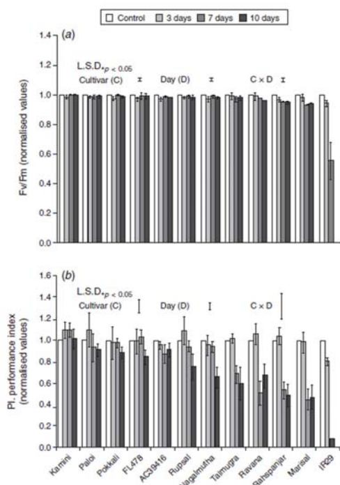
Fig. 6.2: Normalized values (salinity/control) of chlorophyll a fluorescence parameters F_v/F_m and PI_{ABS} in 1 st fully expanded leaf from top on different days after salinity (12 dSm^{-1} ) treatment; Data for IR29 are not available on day 10 of salinity treatment due to the complete mortality. Values are mean of wet and dry seasons. Bar represents S.E.; L.S.D.
