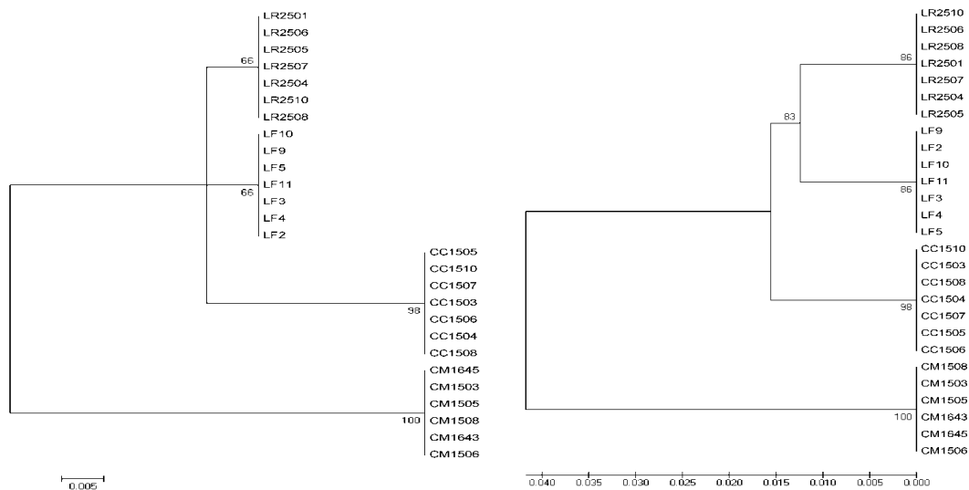
Fig. 2. Phylogenetic trees- NJ (left) and UPGMA (right) of mitochondrial ATPase 8 gene in rohu (LR), catla (CC), mrigal (CM) and fimbriatus (LF). The numbers at nodes indicate percent bootstrap values considering 50% majority rule consensus with 1000 replications.
