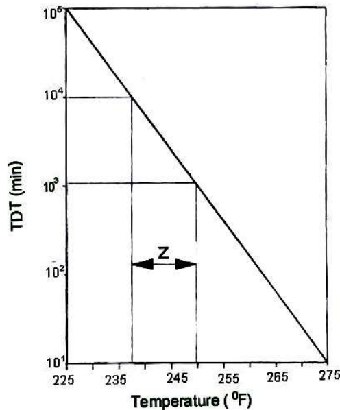
Fig. 2 TDT Curve
