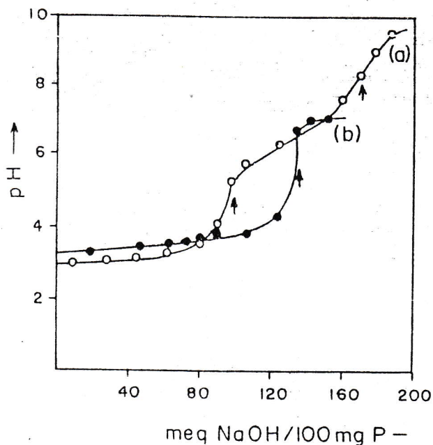
Figure 1. Titration curves of polyphosphoric acid; (a) titration 1; (b) titration 2.
