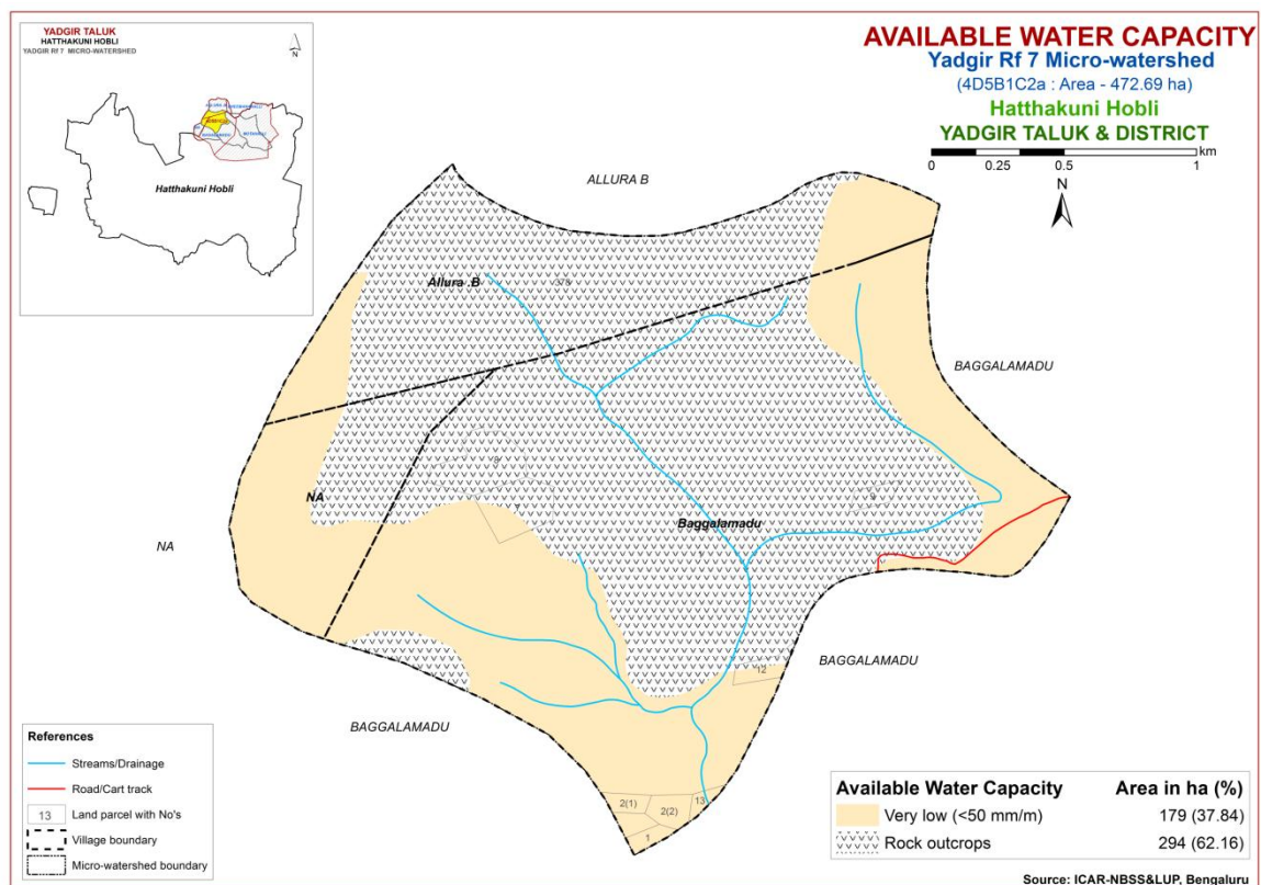
Fig. 5.5 Soil Available Water Capacity map of Yadgir Rf-7 Microwatershed
