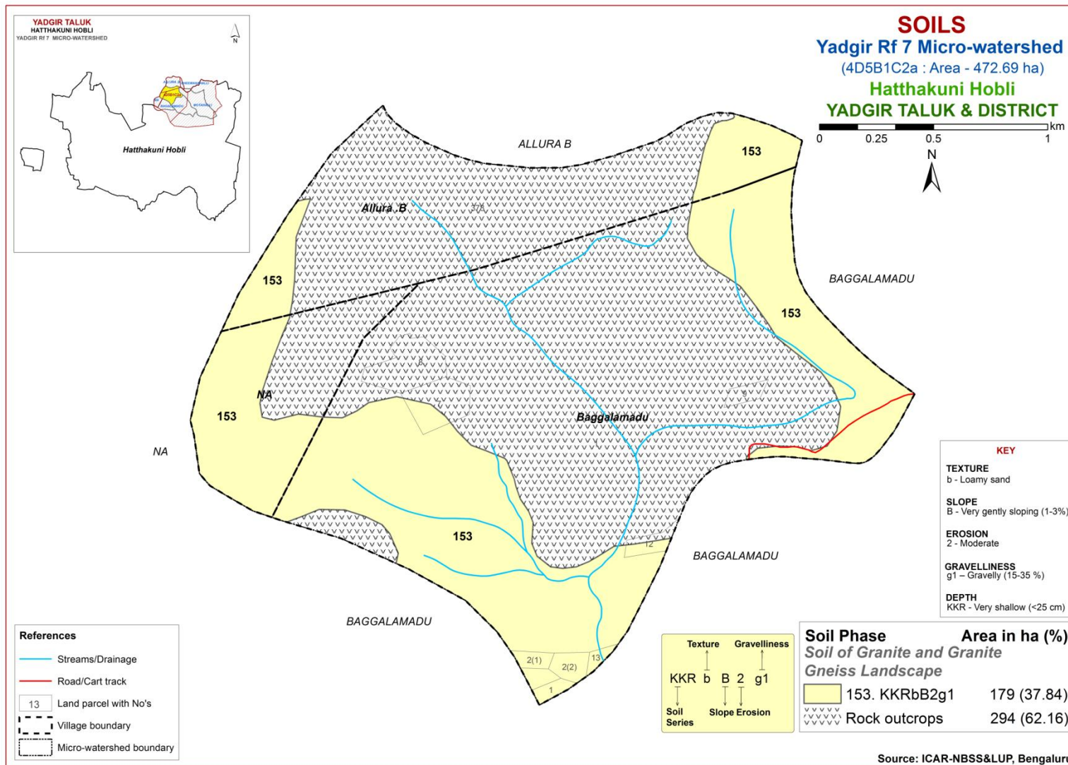
Fig 3.5 Soil Phase or Management Units - Yadgir Rf-7 Microwatershed
