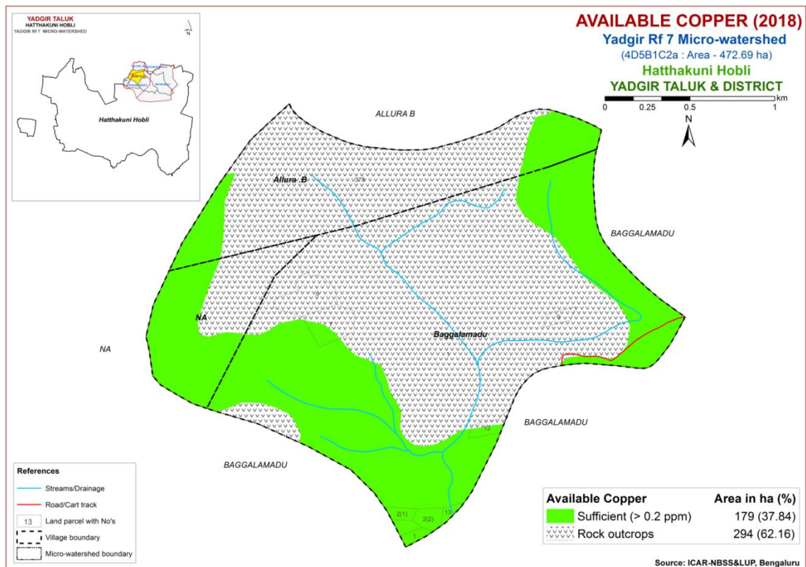
Fig.6.10 Soil Available Copper map of Yadgir Rf-7 Microwatershed
