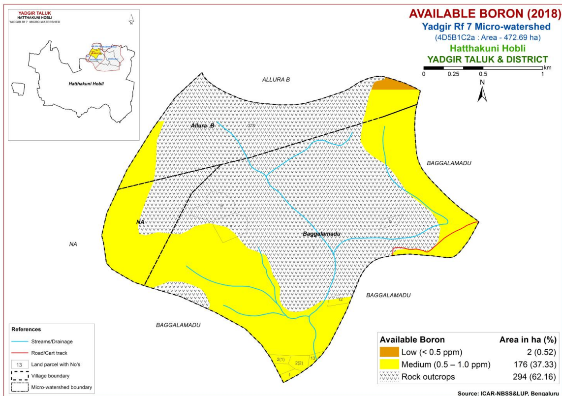
Fig.6.7 Soil Available Boron map of Yadgir Rf-7 Microwatershed
