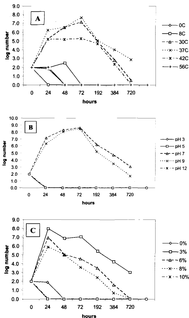
Fig. 4. Growth and survival of urease negative Vibrio parahaemolyticus (MTCC - 451) (A: Temperature, B: pH and C: Salinity).
