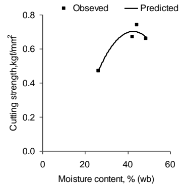
Fig-5 Relationship between cutting strength of henna stem and its moisture content
