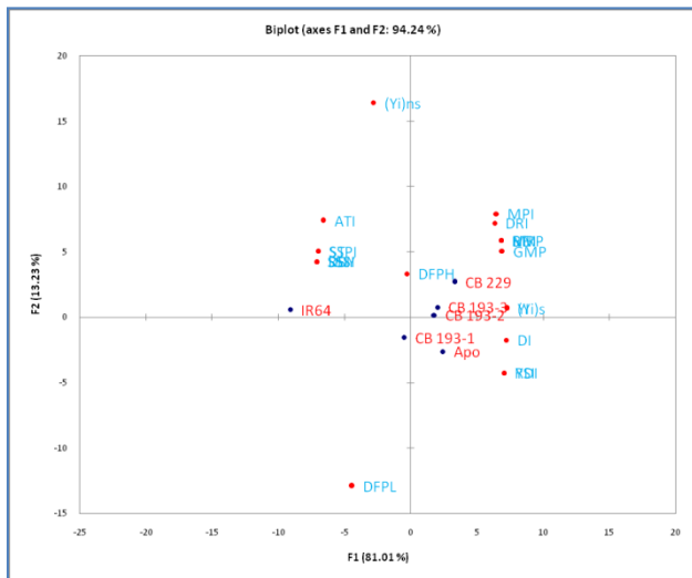
Fig-1 Graphical bi-plot display of stress indices and genotypes evaluated under stress condition
