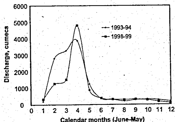
Fig. 2. Hydrograph at Mandleshwar stream gauging station in Narmada basin.
