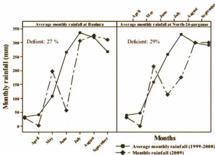
Figure 4. Averages rainfall distribution during 1999-08 compare with 2009 for deficit in rainfall of Bankura and North 24 Parganas districts of West Bengal. Reproduced from (Ref. No 21).
