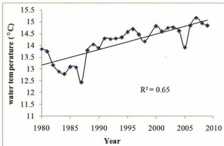
Figure 2. Annual trend in mean minimum water temperature at Haridwar (1980-2009) Reproduced from ( Ref. No 21)
