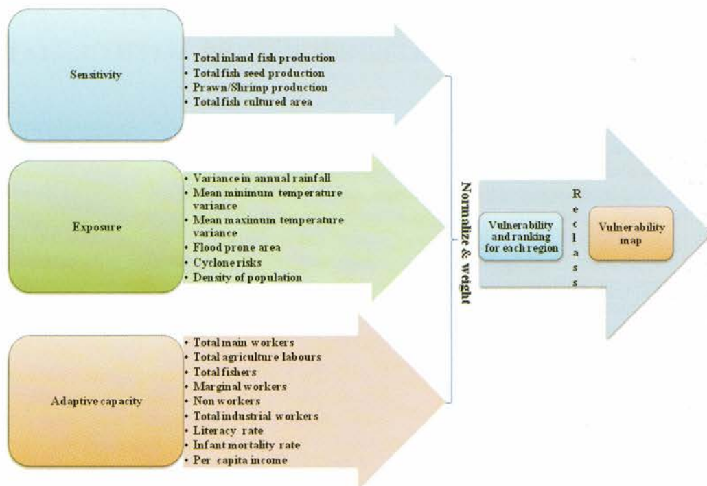
Fig.11 Construction of vulnerability Index Reproduced from (Ref. No 19)
