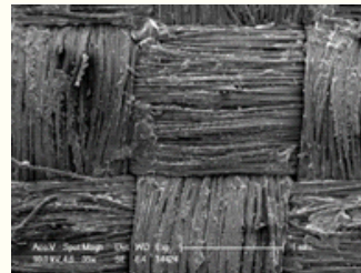
Surface of control fabric after peel strength test
