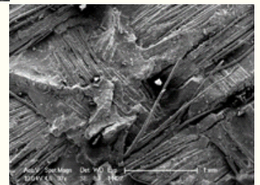
Surface of treated fabric after peel strength test (with rubber deposition)
