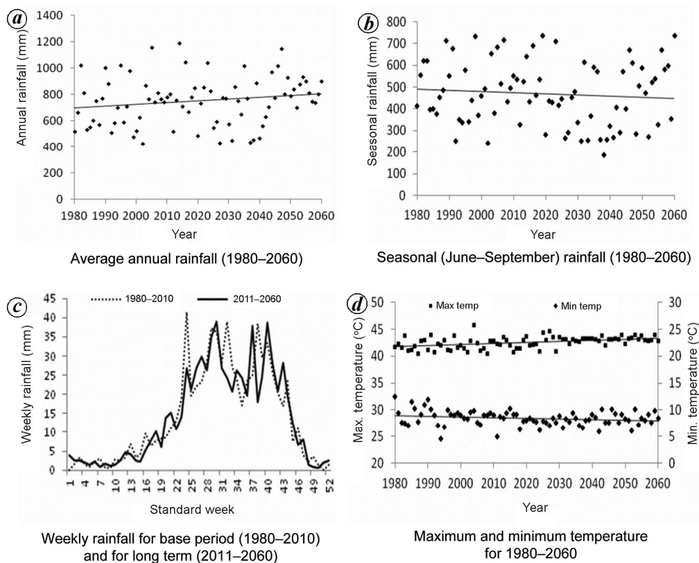
Figure 5. Trend analysis of (a) average annual rainfall, (b) seasonal rainfall, (c) weekly rainfall and (d) air temperature for Yacharam mandal.
