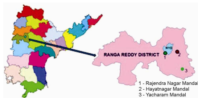
Figure 1. Location map of study mandals in Ranga Reddy district of southern Telangana.
