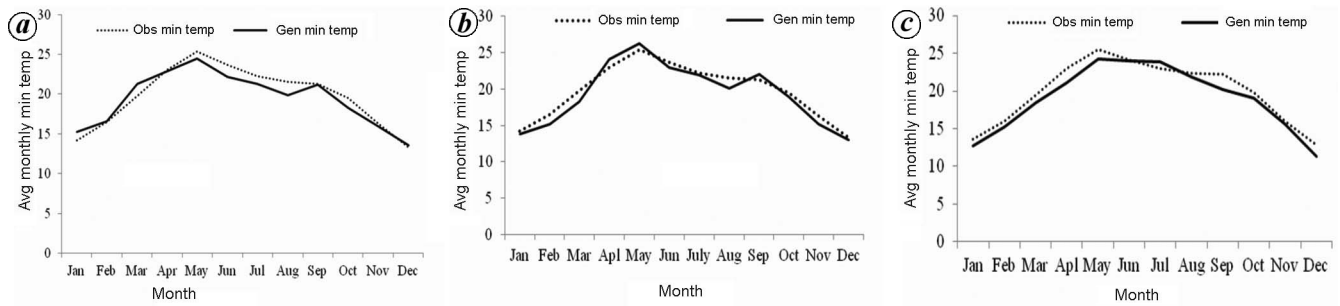
Figure 3. Comparison of monthly observed minimum temperature and generated minimum temperature: a , Yacharam; b , Hayathnagar; c , Rajendranagar (1980–2010).
