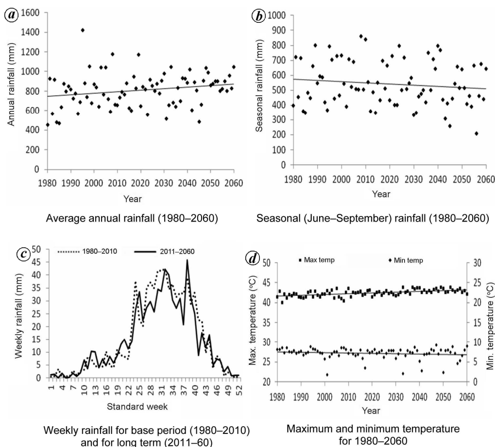
Figure 7. Trend analysis of (a) average annual rainfall, (b) seasonal rainfall, (c) weekly rainfall and (d) air temperature for Rajendranagar mandal.
