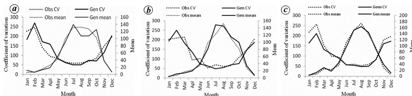
Figure 2. Comparison of observed and generated mean and coefficient of variation of monthly rainfall: a , Yacharam; b , Hayathnagar; c , Rajendranagar (1980–2010).
