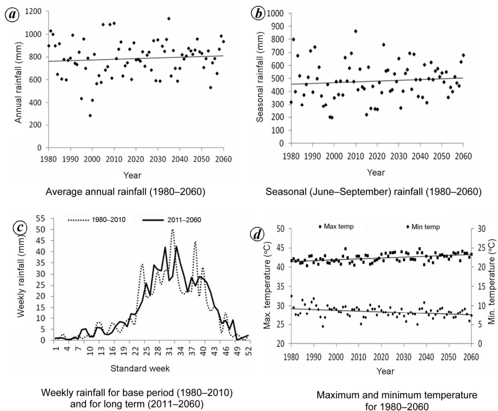
Figure 6. Trend analysis of (a) average annual rainfall, (b) seasonal rainfall, (c) weekly rainfall and (d) air temperature for Hayathnagar mandal.
