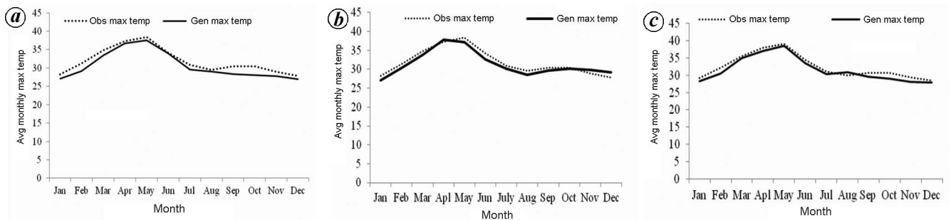
Figure 4. Comparison of monthly observed maximum temperature and generated maximum temperature: a , Yacharam; b , Hayathnagar; c , Rajendranagar (1980–2010).
