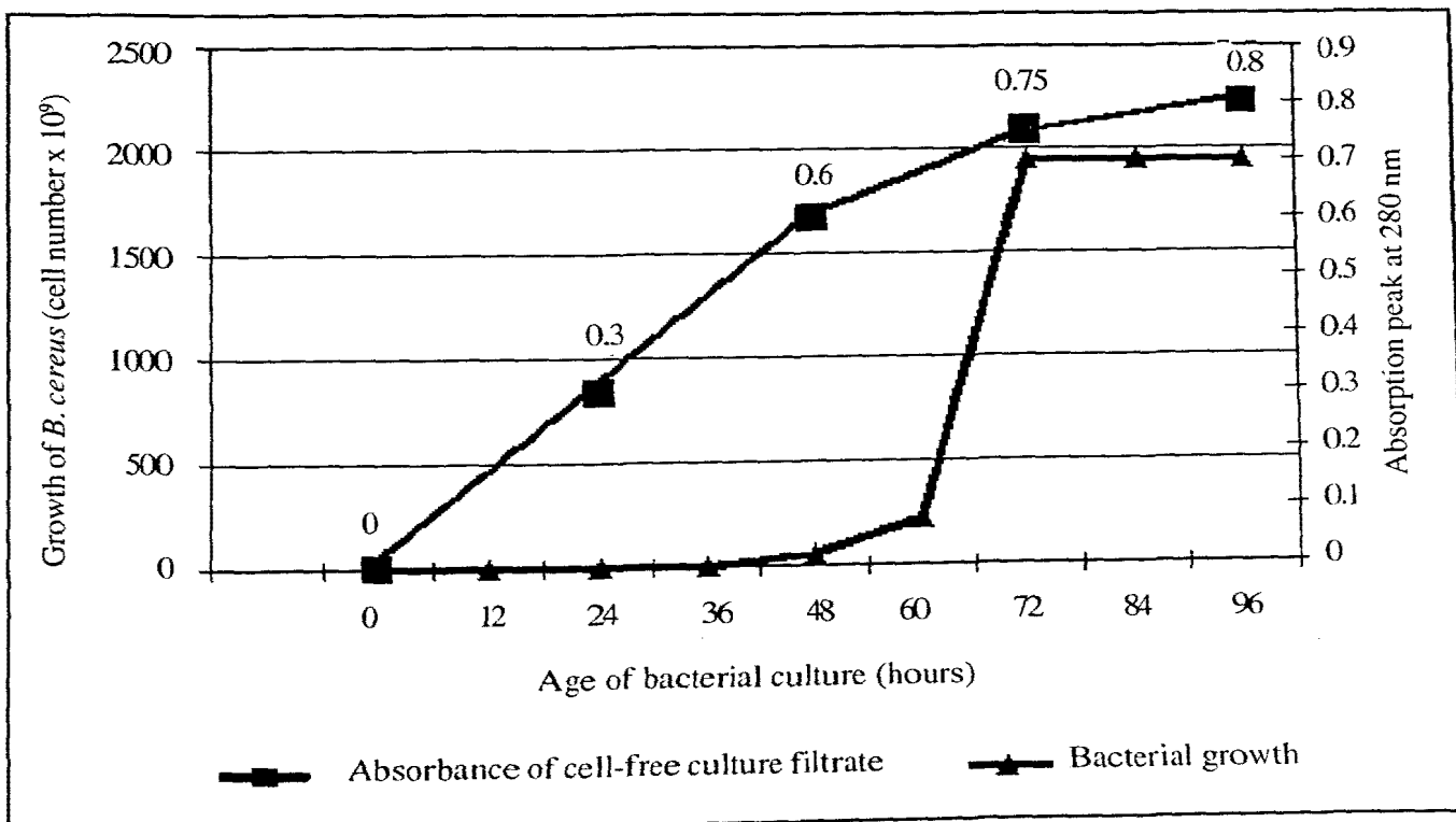
Figure 1. Absorbance peaks of B. cereus cells during growth phase and cell-free culture filtrates
