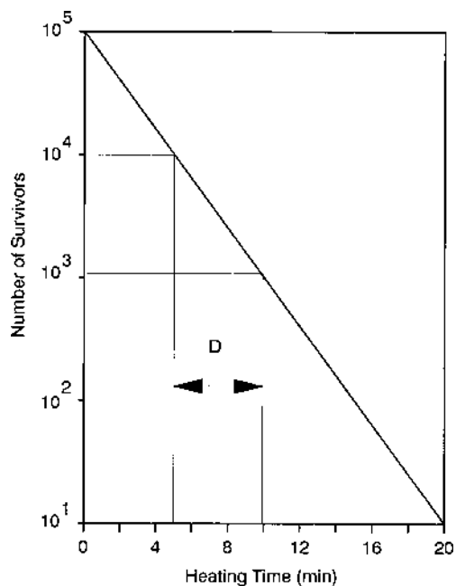
Fig 1. Survivor curve
