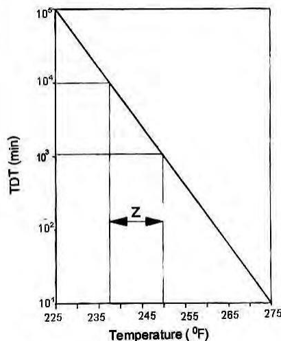
Fig. 2 TDT Curve
